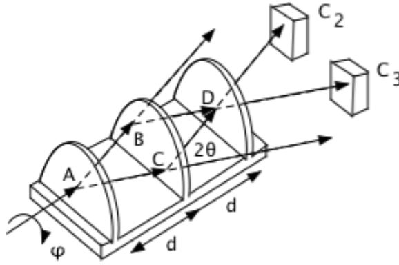
Figure 13.5: Experimental Setup
