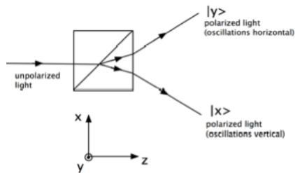
Figure 11.22: Wollaston Prism - Polarizer
