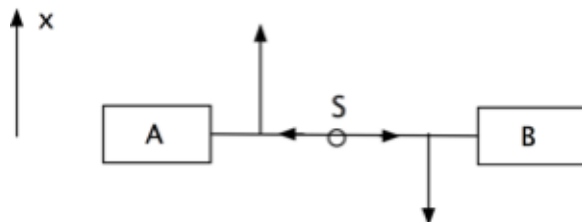
Figure 11.17: EPR Scenario
