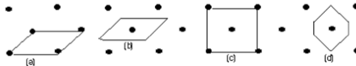
Figure 14.5: Primitive Cells
