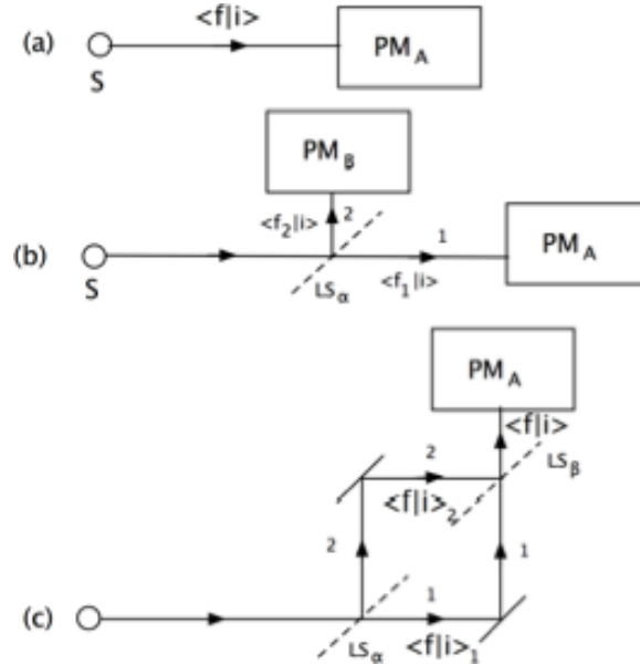
Figure 11.14: Three Arrangements
