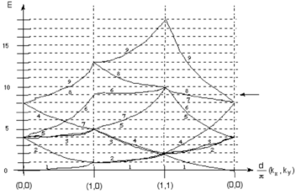
Figure 14.60: Step #7
