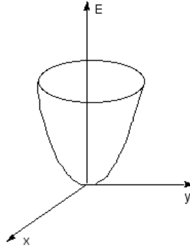
Figure 14.48: E(k) paraboloid
