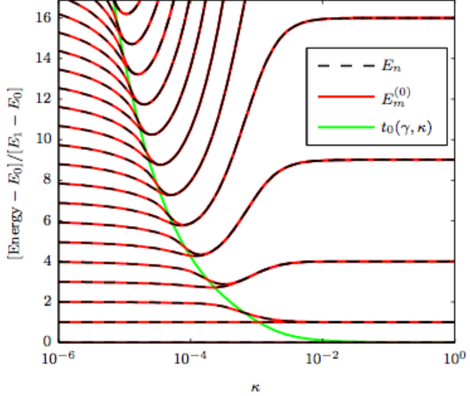
Figure 14.79: Exact and approximate energies as a function of \kappa for \gamma = -10 . The black dashed curves show the exact energies E_n , while the solid red curves show the approximate energies E_m^{(0)} found from the lowest potential-curve in the second Born-Oppenheimer equation. The green curve shows the position of the maximum of the lowest potential curve \epsilon_0(q_+) within the perturbative approximation. The exact ground state energy E_0 , which varies with \kappa , has been subtracted from all energies, and afterward, the energies is scaled by the energy difference between the two lowest exact energy levels E_1 - E_0 .
