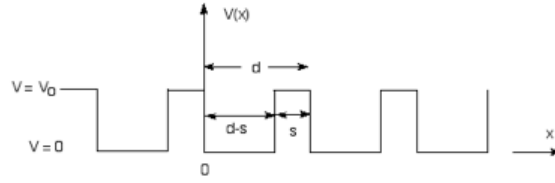
Figure 14.80: Piecewise Constant Potential - 1 Atom per Primitive Cell
