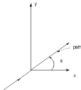
Figure 14.49: Path in k space
