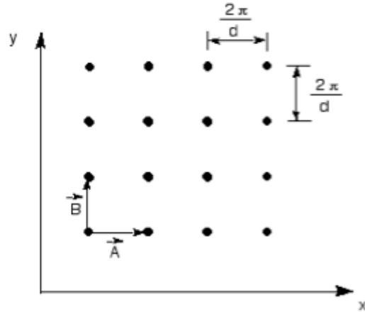
Figure 14.19: Reciprocal Lattice for Square direct lattice
