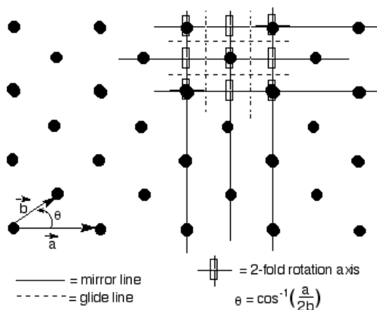
Figure 14.8: Centered Rectangular Lattice
