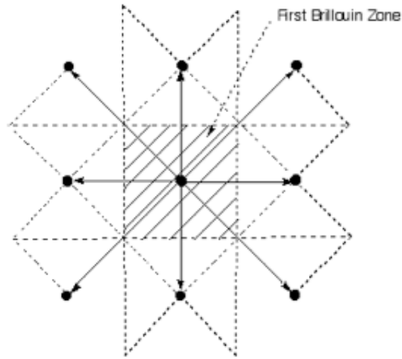
Figure 14.22: Construction of first zone
