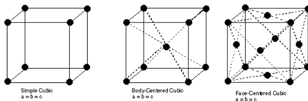
Figure 14.14: 3-Dimensional Crystals
