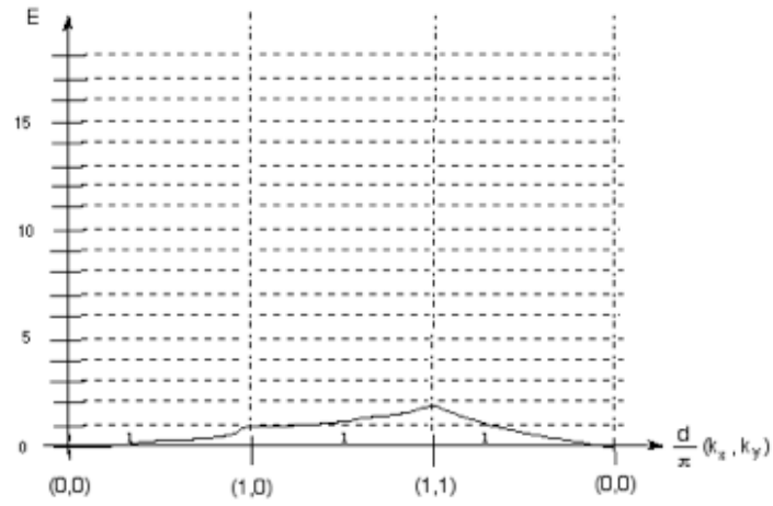
Figure 14.54: Step #1
