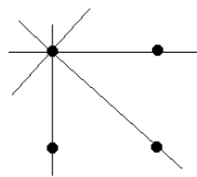
Figure 14.11: Mirror Lines in Square Lattice
