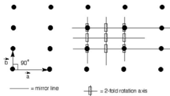
Figure 14.7: Primitive Rectangular Lattice
