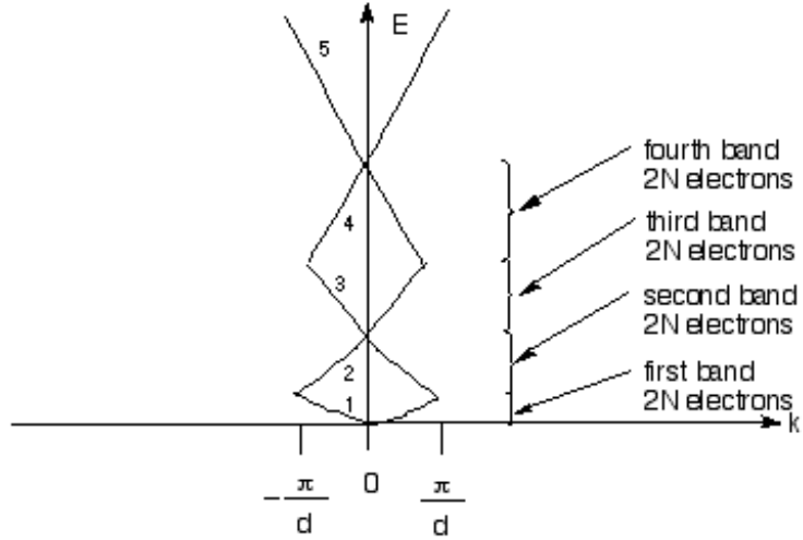
Figure 14.32: E versus k - Final Plot in Reduced Zone Scheme
