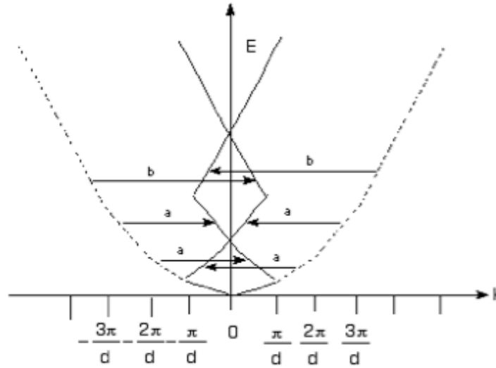
Figure 14.31: E versus k - Reduced Zone Scheme
