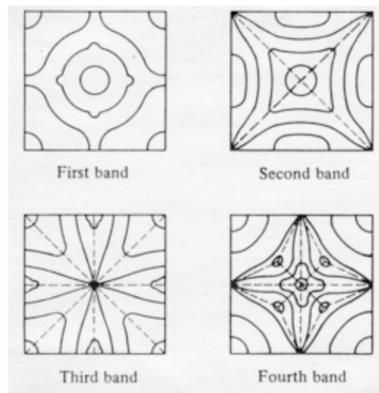
Figure 14.73: Modified constant energy contours
