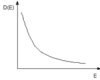
Figure 14.33: Density of states D(E)
