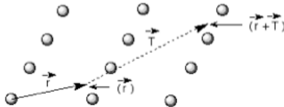
Figure 14.3: Translation Invariance
