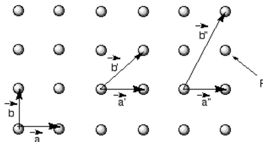
Figure 14.4: Alternate Basis Vectors
