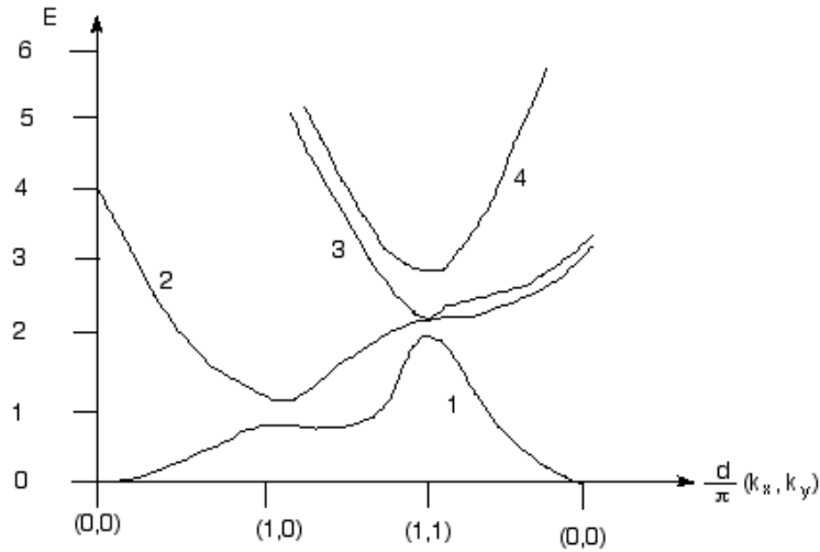
Figure 14.71: Band Gaps create Distinct Bands
