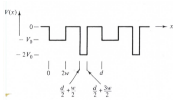
Figure 14.81: Piecewise Constant Potential - 2 Atoms per Primitive Cell
