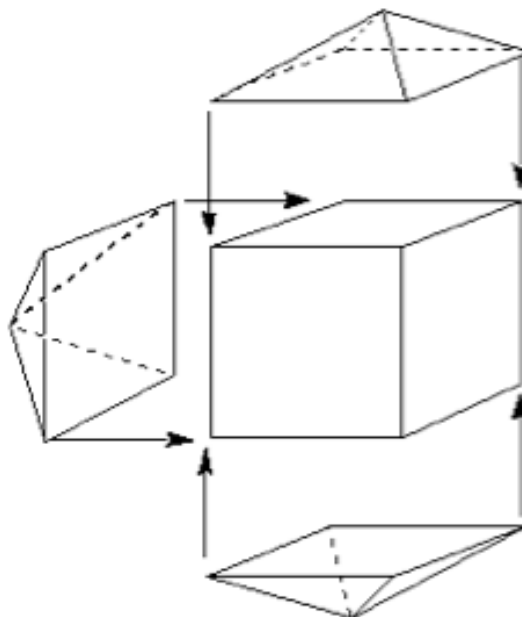
Figure 14.28: Parts of the Second Brillouin zone
