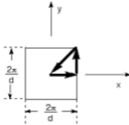
Figure 14.52: Path in k space through high symmetry points
