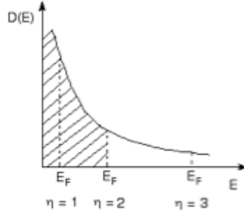
Figure 14.37: Occupied states on D(E) plot - Various \eta values
