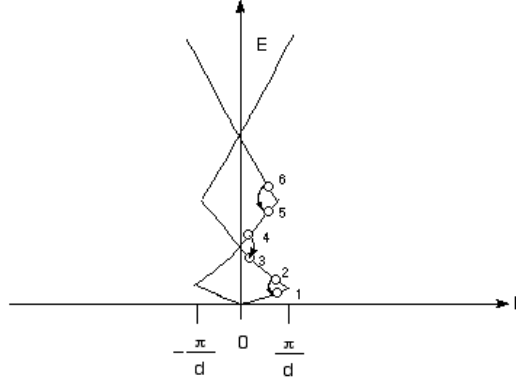
Figure 14.39: Strongly mixed states in Reduced Zone Scheme
