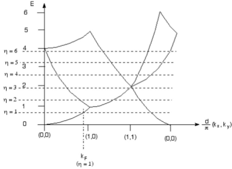
Figure 14.69: First 4 bands with location of Fermi surfaces
