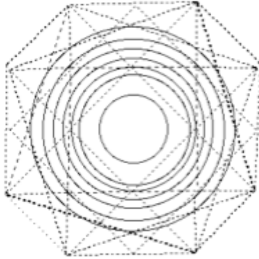
Figure 14.67: Fermi surfaces
