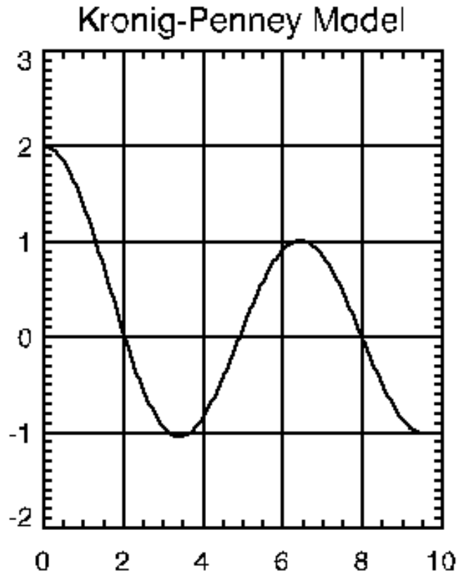
Figure 14.46: Kronig-Penney Model - Transcendental Plot
