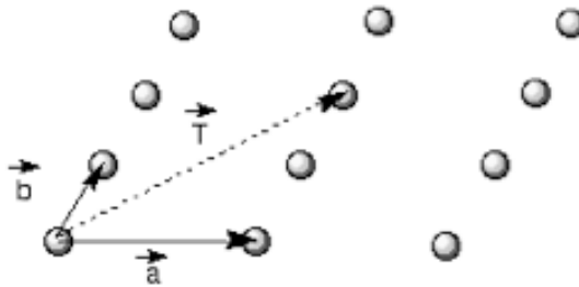
Figure 14.2: 2-dimensional crystal
