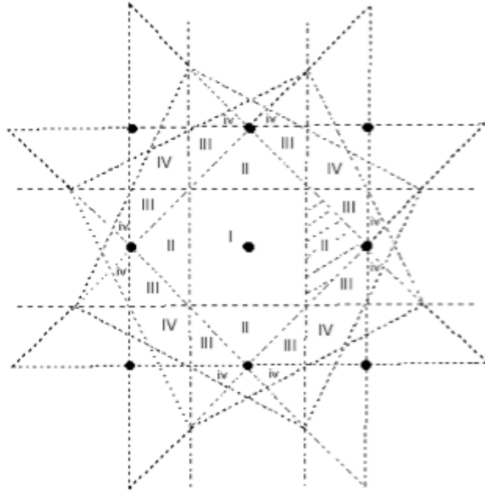
Figure 14.23: Construction of higher zones
