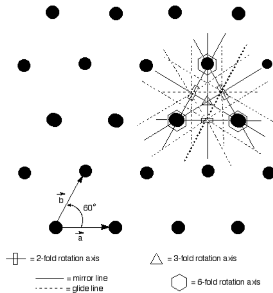
Figure 14.10: Hexagonal Lattice
