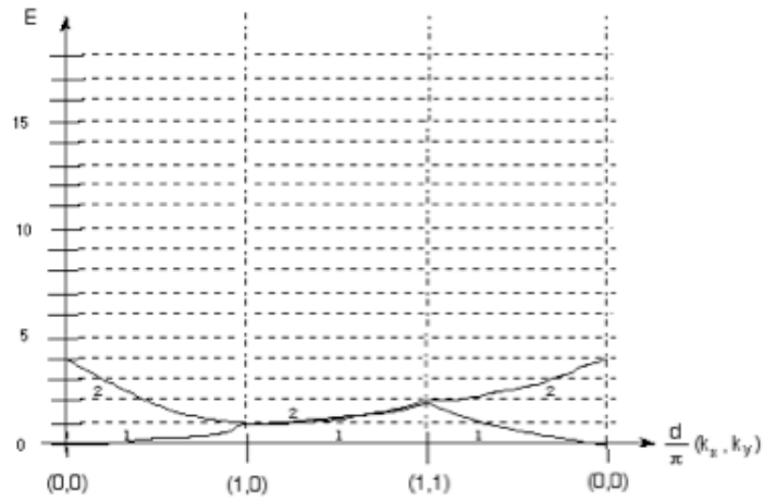
Figure 14.55: Step #2
