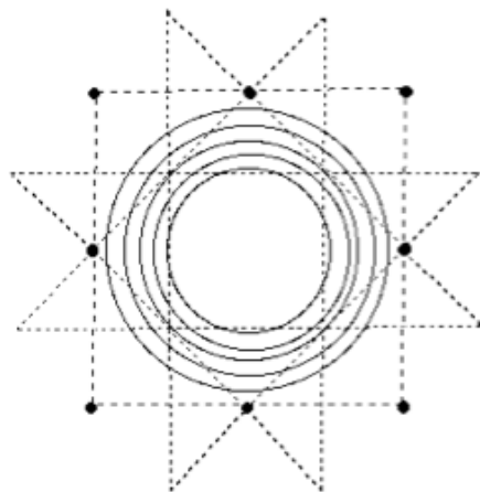
Figure 14.64: Energy contours in extended scheme
