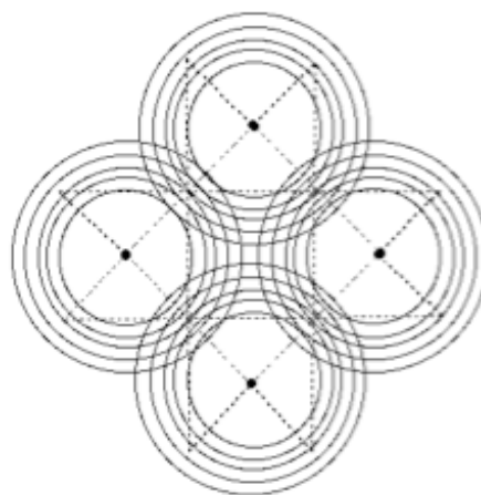
Figure 14.65: Translating contours to second band regions
