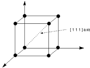
Figure 14.15: [111] axis in cubic lattice
