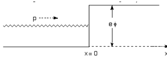
Figure 15.1: Electrostatic Potential Barrier - Klein Paradox
