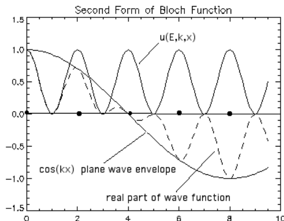
Figure 14.17: Second form of Bloch function
