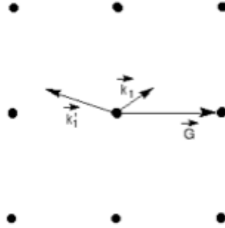
Figure 14.20: |\vec{k}'_1| > |\vec{k}_1|
