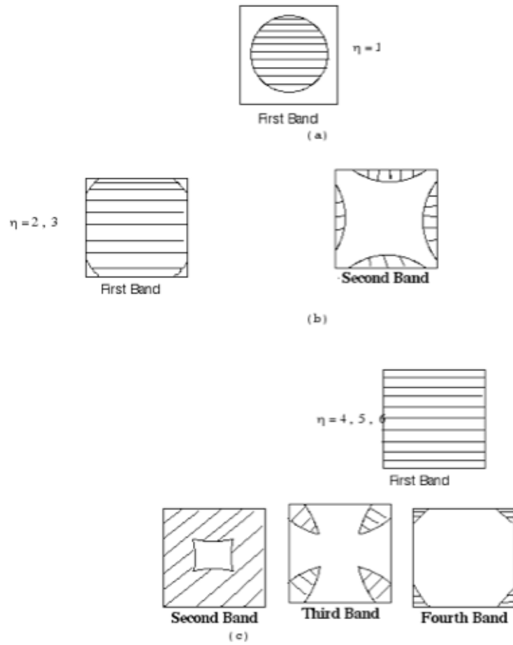
Figure 14.68: Fermi surfaces translated to first zone
