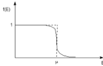
Figure 14.34: Fermi-Dirac Distribution Function
