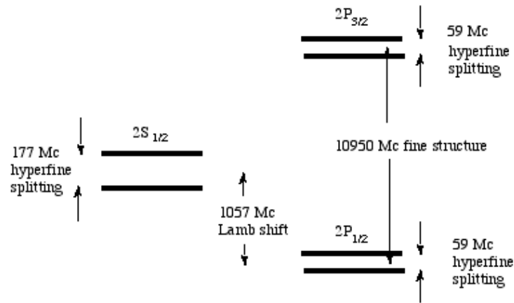
Figure 15.4: n = 2 Energy level structure for relativistic hydrogen
