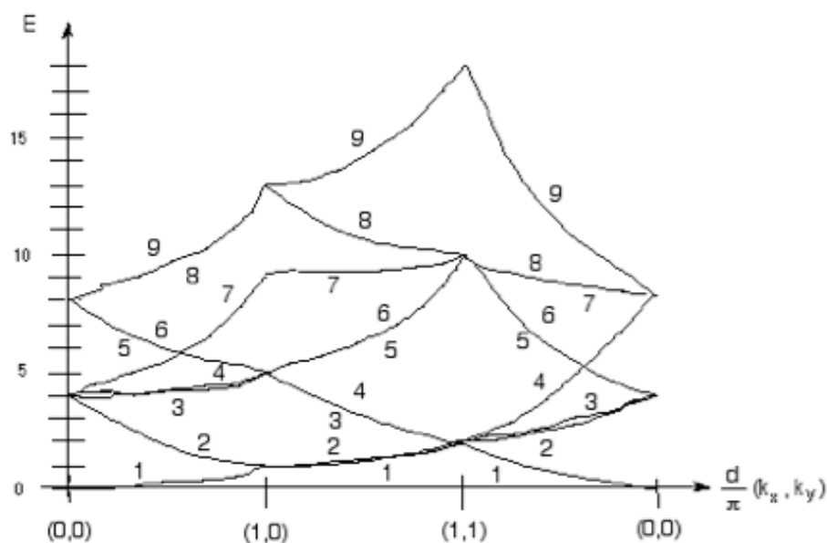
Figure 14.61: First 9 Bands
