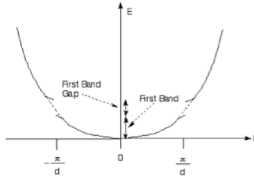
Figure 14.41: Band Gaps in Extended Zone Scheme
