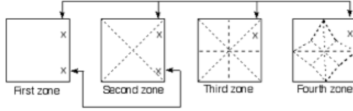
Figure 14.70: Strongly mixing states
