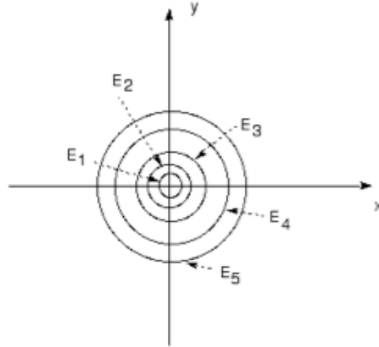
Figure 14.51: Constant energy contours in k space
