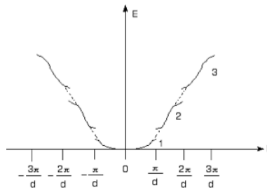
Figure 14.43: Band Gaps in Extended Zone Scheme
