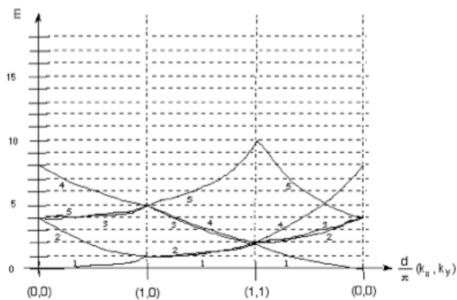
Figure 14.58: Step #5
