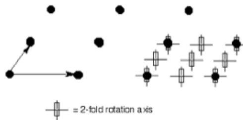
Figure 14.6: Oblique Lattice
