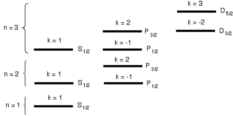
Figure 15.3: Energy level structure for relativistic hydrogen
