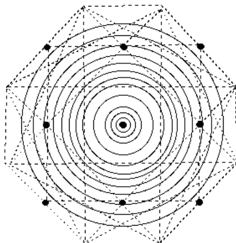
Figure 14.62: First 7 zones with energy contours - square lattice
