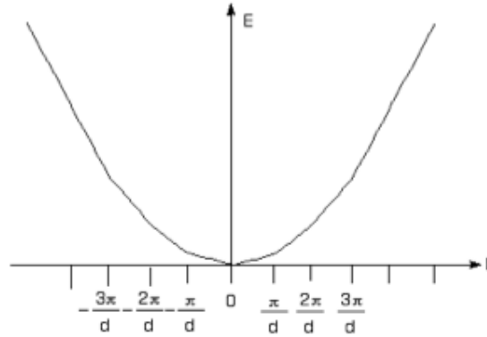
Figure 14.30: E versus k - Extended Zone Scheme
