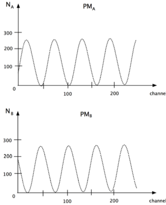
Figure 11.13: Interference Results
