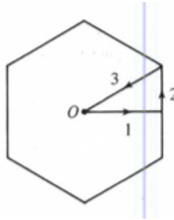
Figure 14.83: Paths in the First Brillouin Zone
