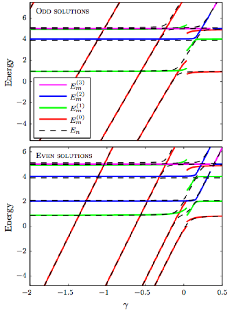
Figure 14.78: Exact and approximate energies as a function of \gamma for \kappa = 1 . Exact energies are plotted by the black dashed lines, and for n = 0, 1, 2, 3 the energies E_j^{(n)} found from the Born-Oppenheimer equation is plotted in four different colors.
