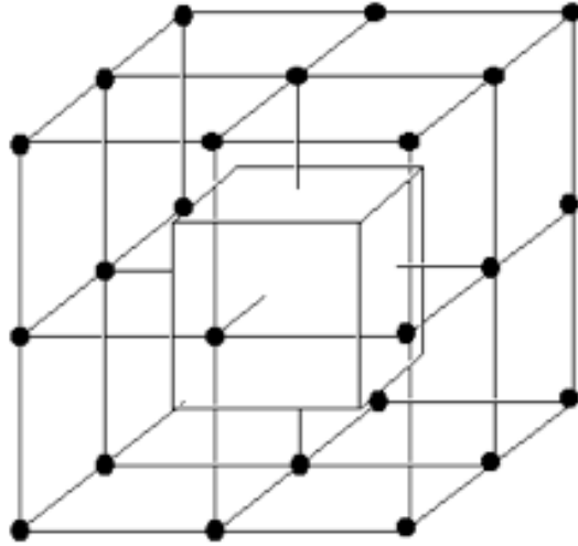
Figure 14.26: First Brillouin zone of Simple Cubic Lattice
