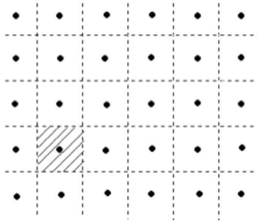
Figure 14.24: First Brillouin zone as primitive cell
