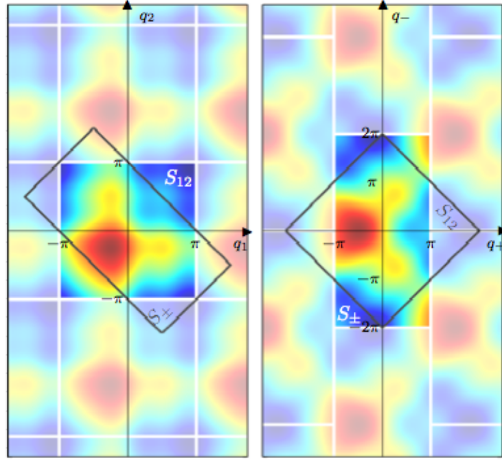
Figure 14.75: Quasi-momentum of the two particles vs. relative and center-of-mass quasi-momentum. Left: The first Brillouin zone S_{12} in the (q_1, q_2) -plane is emphasized and repeated in each direction. The color coding indicates the values of a function that is periodic in both variables with period 2\pi and illustrates the required periodicity. The set S_{\pm} which contains exactly one representative of each point from S_{12} is shown by the gray rectangle. Right: The same function is shown but in the (q_+, q_-) -coordinate system. The set S_{\pm} is emphasized and repeated, but with a different tiling than for S_{12} in the left panel.
