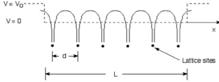
Figure 14.29: Free Electron Approximation
