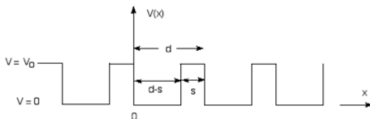
Figure 14.45: Kronig-Penney Potential
