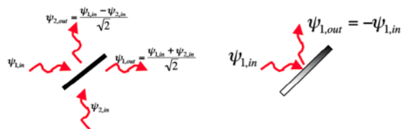
Figure 11.10: Input/output Transformations
