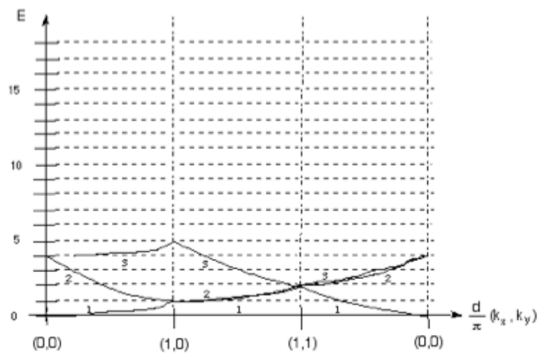
Figure 14.56: Step #3
