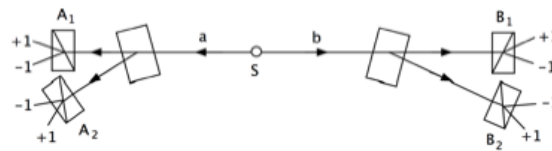
Figure 11.27: Second Orsay Experiment using Optical Switches
