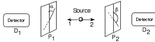
Figure 11.3: Bell-EPR Experiment
