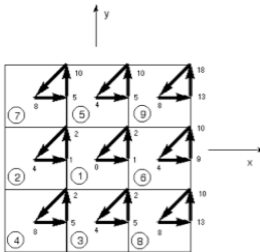
Figure 14.53: Equivalent paths in k space by translation
