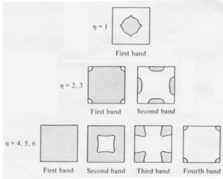
Figure 14.74: Fermi surfaces for \eta = 1
