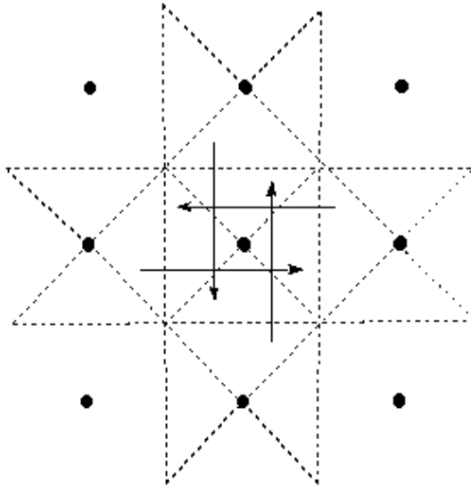
Figure 14.25: Translating higher zone to first zone
