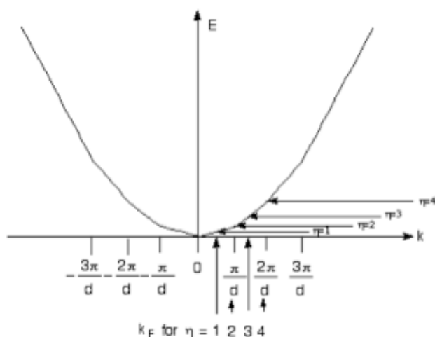
Figure 14.35: Fermi Energy in Extended Zone Scheme - Various \eta values
