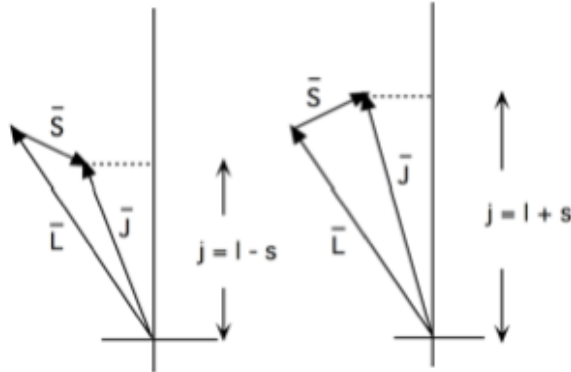
Figure 13.3: Extreme Orientations
