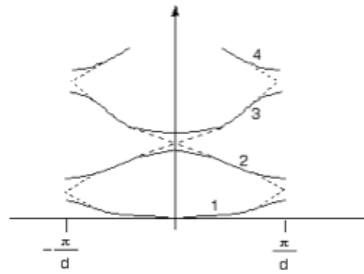
Figure 14.42: Band Gaps in Reduced Zone Scheme
