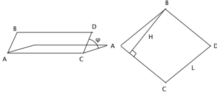
Figure 13.7: Geometrical Considerations
