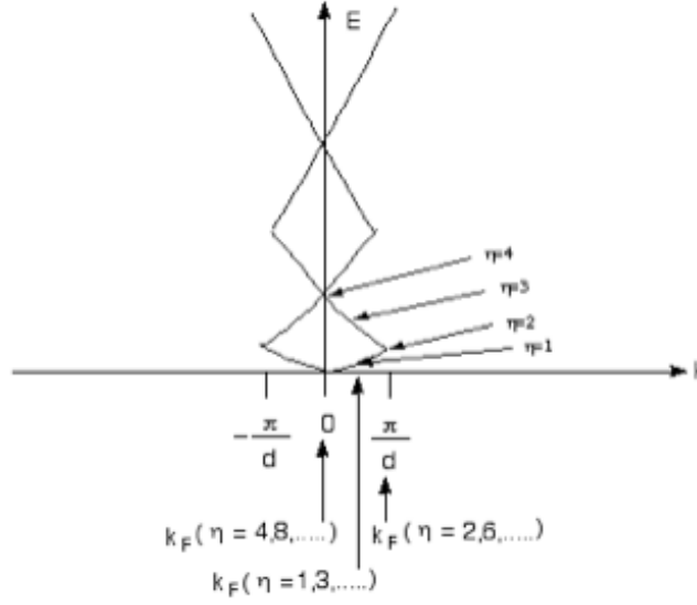
Figure 14.36: Fermi Energy in Reduced Zone Scheme - Various \eta values
