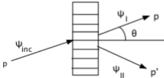
Figure 13.6: Splitting Waves
