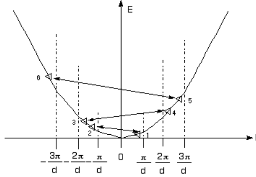
Figure 14.38: Strongly mixed states in Extended Zone Scheme
