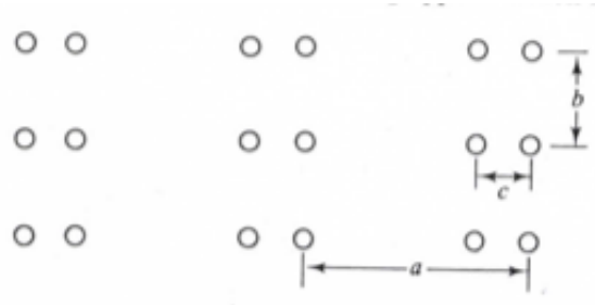
Figure 14.84: 2-Dimensional Crystal - Rectangular Bravais Lattice with 2 Atoms per Primitive Unit Cell
