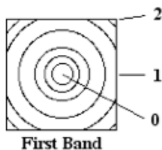
Figure 14.63: Energy contours in first band
