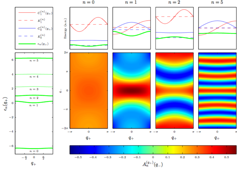
Figure 14.76: Energies and eigenfunctions found by solving the two Born-Oppenheimer equations for \kappa = 0.5 and \gamma = -0.5 . Left panel: The six lowest potential curves \epsilon_n(q_+) found from the first Born-Oppenheimer equation. Upper panels: Magnification of four of the potential curves in the left panel. Lower panels: Eigenfunctions A_n^{(q_+)}(q_-) for the first Born-Oppenheimer equation shown for all values of q_+ for the corresponding n -values. In the upper panels are shown (horizontal dashed blue/red lines) the two lowest energies E_j^{(n)} for j = 1, 2 found from solving the second Born-Oppenheimer equation in the potential \epsilon_n(q_+) and the corresponding wave functions (solid blue/red lines).
