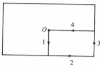
Figure 14.82: Paths in the First Brillouin Zone
