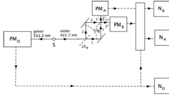
Figure 11.12: Mach-Zehnder Interferometer Inserted
