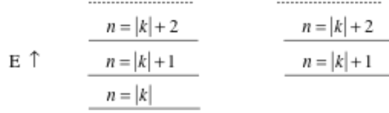
Figure 15.2: Dirac hydrogen energy level structure
