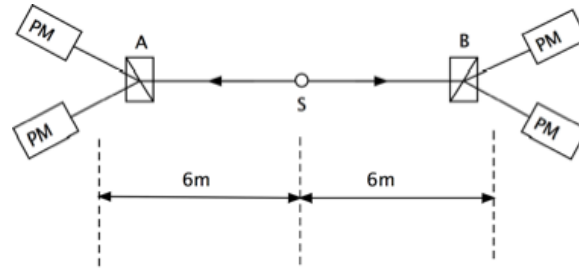
Figure 11.25: Orsay Experiment - Details
