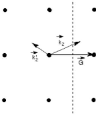
Figure 14.21: |\vec{k}'_1| > |\vec{k}_1|
