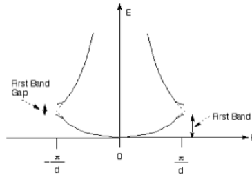
Figure 14.40: Band Gaps in Reduced Zone Scheme
