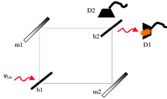
Figure 11.11: Mach-Zehnder Interferometer
