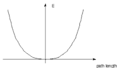
Figure 14.50: E versus path in k space
