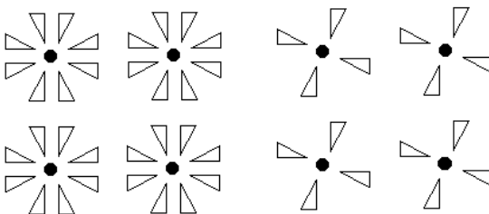
Figure 14.13: Possible Crystals
