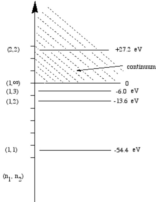
Figure 12.4: Helium Energy level Spectrum
