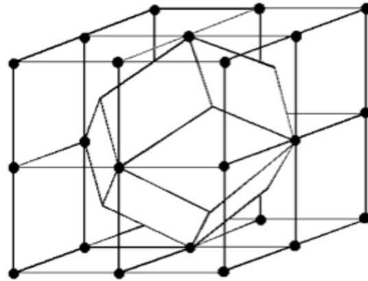
Figure 14.27: Second Brillouin zone of Simple Cubic Lattice
