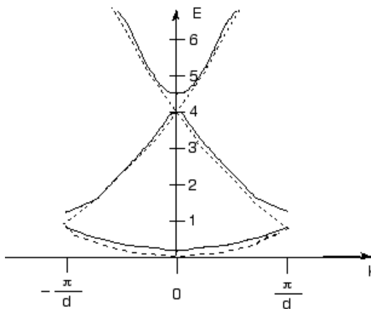
Figure 14.47: Energy Bands and Gaps in the Kronig-Penney Model
