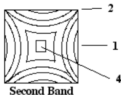
Figure 14.66: Energy contours in second band
