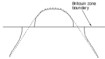
Figure 14.72: Constant energy contours bending toward zone boundaries
