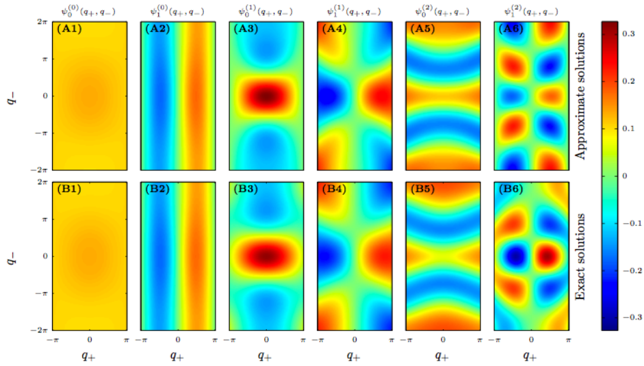
Figure 14.77: Upper panels: Quasi-momentum wave functions found by the Born-Oppenheimer approximation for \kappa = 0.5 and \gamma = -0.5 . Columns 1-2 show the two lowest eigenstates in the lowest potential curve \epsilon_0(q_+) corresponding to the n = 0 column in figure 14.76. Columns 3-4 correspond to the n = 1 column in figure 14.76 and columns 5-6 correspond to the n = 2 column in figure 14.76. Lower panels: The corresponding exact solutions.
