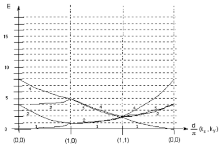
Figure 14.57: Step #4
