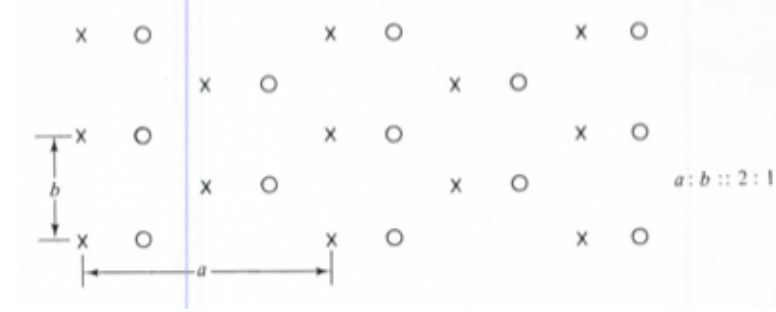
Figure 14.85: 2-Dimensional Crystal - Centered Rectangular Bravais Lattice with 2 Atoms per Primitive Unit Cell
