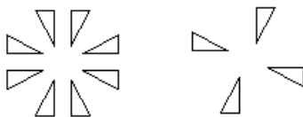
Figure 14.12: Possible Bases
