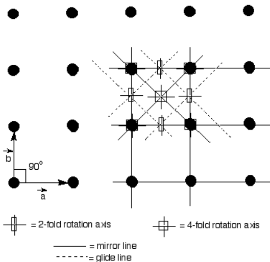
Figure 14.9: Square Lattice
