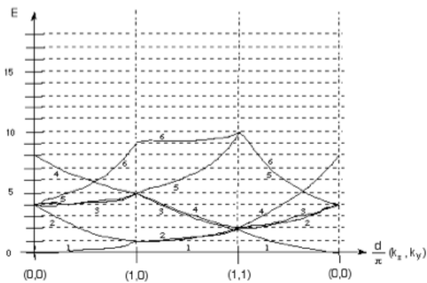
Figure 14.59: Step #6
