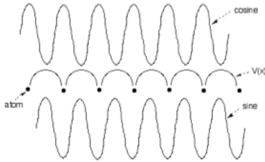
Figure 14.44: Probability Densities
