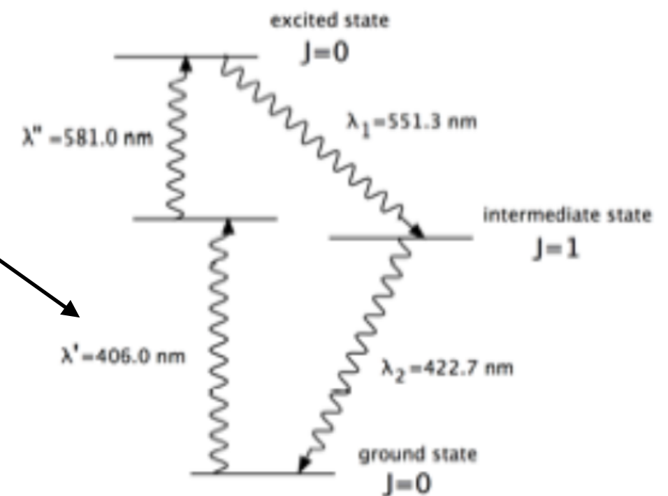
Calcium based light source - Energy Levels
